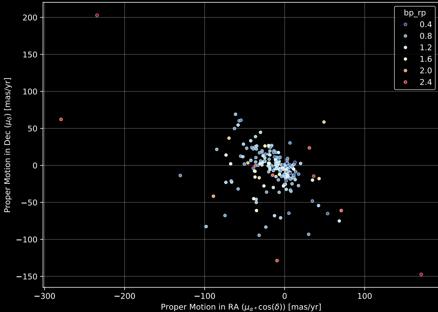
APOGEE DR17 Field: [098+60_MGA] Proper Motion Diagram (n= 200)
