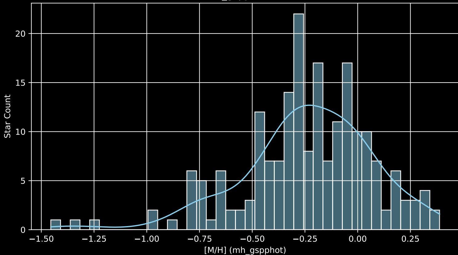
APOGEE DR17 Field: [098+60_MGA [M/H] (mh_gspphot) (n= 200)
