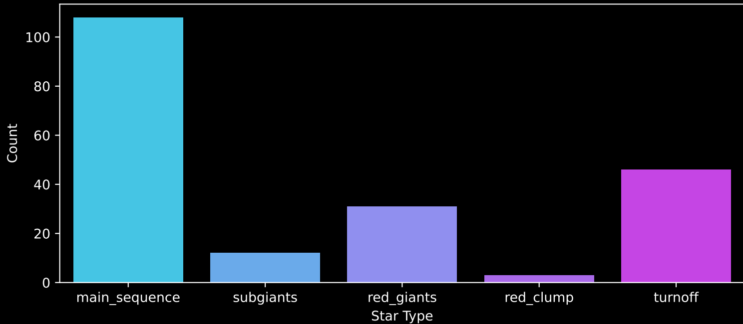
APOGEE DR17 Field: [098+60_MGA] Count plot of Star Type
