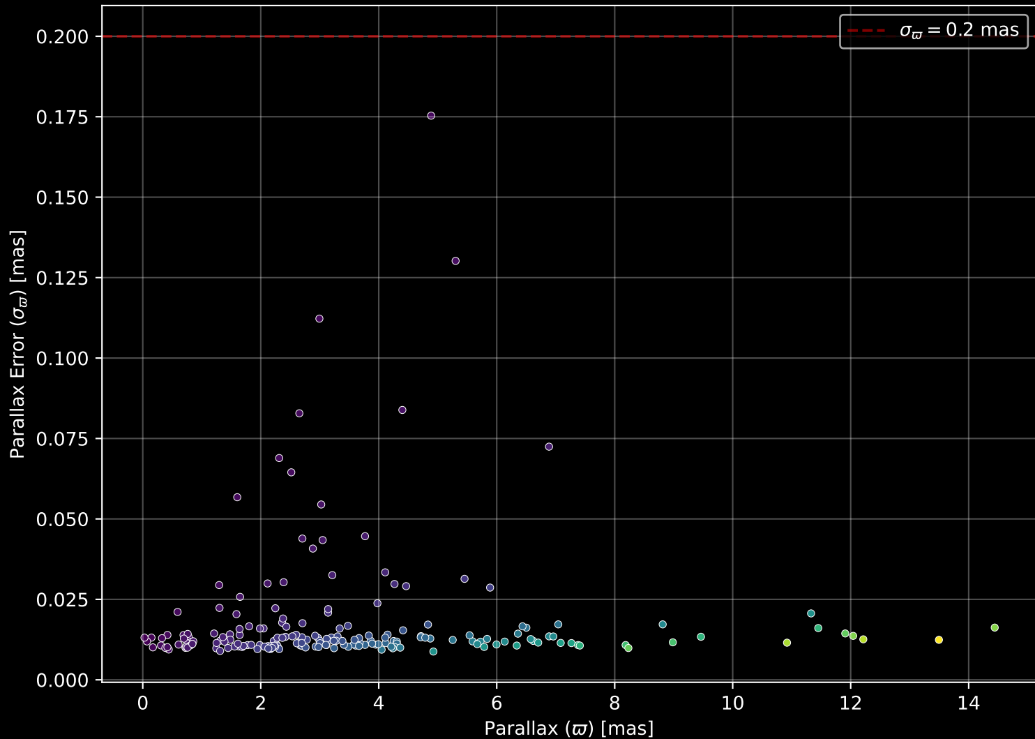
APOGEE DR17 Field: [098+60_MGA] Parallax Quality (n= 200)
