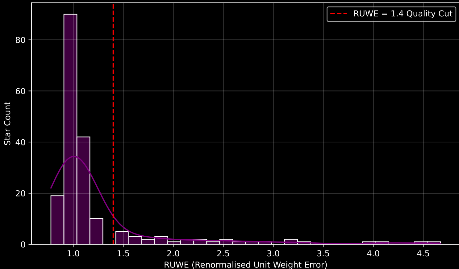
GAPOGEE DR17 Field [098+60_MGA] RUWE Distribution (n= 192)
